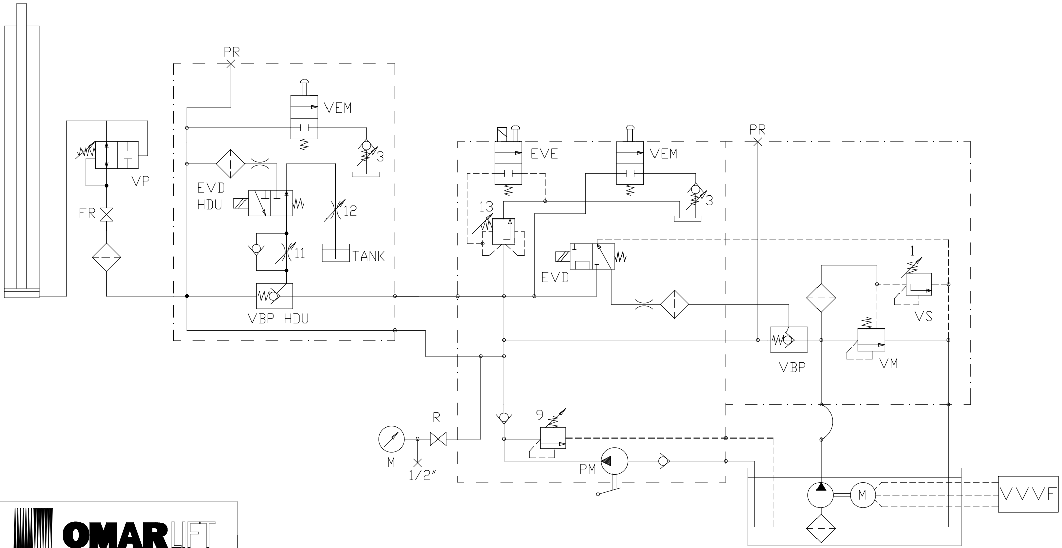
SCHEMA IDRAULICO VALVOLA HI 600+ HDU OMARLIFT - rev.02 13/07/2022 HI 600 VALVE + HDU VALVE OMARLIFT HYDRAULIC SCHEME
